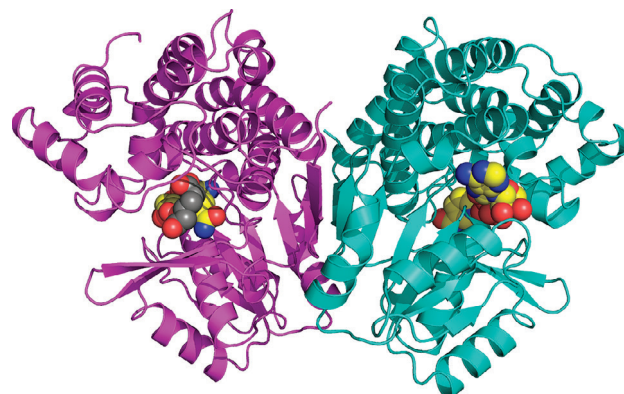
Figure 1. Dimeric molecular structure of GraC-coenzyme-ligand complex.
