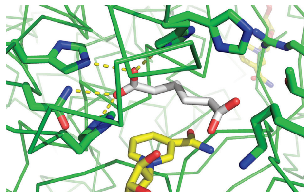
Figure 3. The active-site structure of GraC-coenzyme-ligand complex.
