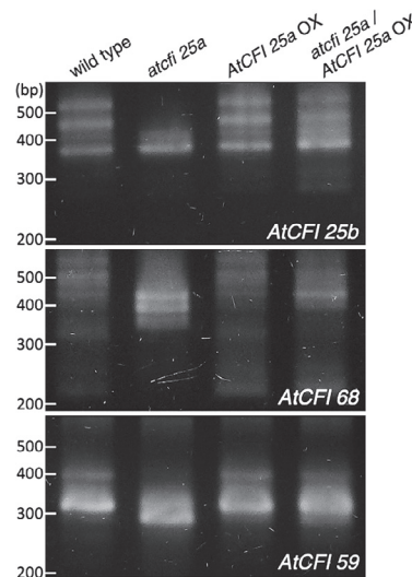
Figure 3. Comparison of cleavage and polyadenylation sites of wild type, atcfi 25a , AtCFI 25a OX , and atcfi 25a-3 / AtCFI 25a OX for genes encoding putative CFI subunits. 3' RACE amplifications of AtCFI 25a , AtCFI 25b , AtCFI 68 , and AtCFI 59 are shown as comparable gel patterns on agarose gel after electrophoresis. Note that the of the 3' UTR length pattern is less diverse in atcfi 25a while those in AtCFI 25a OX and atcfi 25a-3 / AtCFI 25a OX is similar to wild type. Bands were confirmed to represent 3' UTR of each gene through sequencing. Subjected samples: 7 DAS seedlings.
