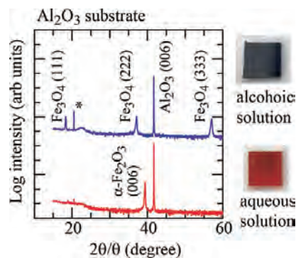
Figure 2. Photographs and X-ray 2 \theta profiles for (upper) Fe 3 O 4 and (lower) \alpha -Fe 2 O 3 films grown on (001) Al 2 O 3 substrates.
