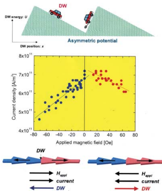
Figure 2. Schematic illustration of the motion of magnetic domain wall in asymmetric potential barriers (top). Magnetic field dependence of the critical current density (middle). Red and blue dots show the values of the critical current density for the rightward and the leftward propagation, respectively. The magnetic structure and the directions of a current and a magnetic field are shown (bottom).
