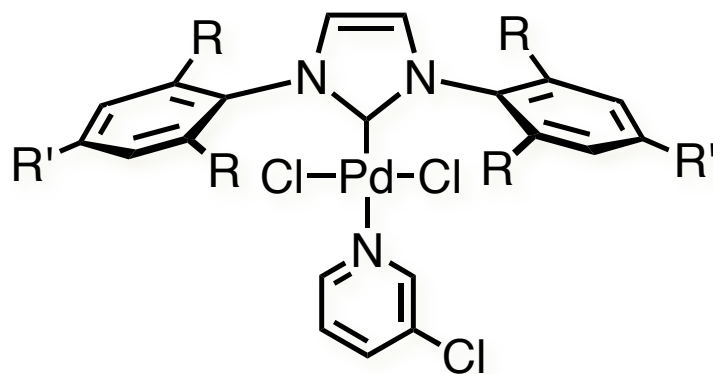
Pd-PEPPSI complex
